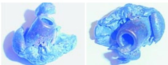
AK47 Slugs after Hitting TERRABRICK at 25 Yards
